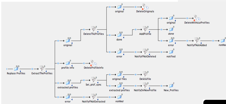
Sample workflow created and displayed with FlowView Pro
